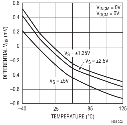
Differential Input Offset Voltage vs Temperature (Note 7)
