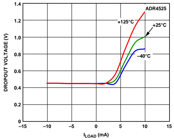
Figure 19. ADR4525 Dropout Voltage vs. Load Current
