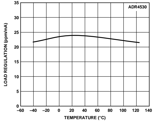
Figure 34. ADR4530 Load Regulation vs. Temperature (Sourcing)
