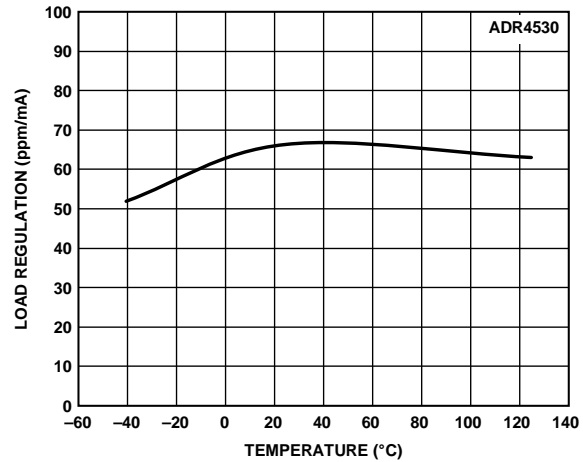
Figure 35. ADR4530 Load Regulation vs. Temperature (Sinking)
