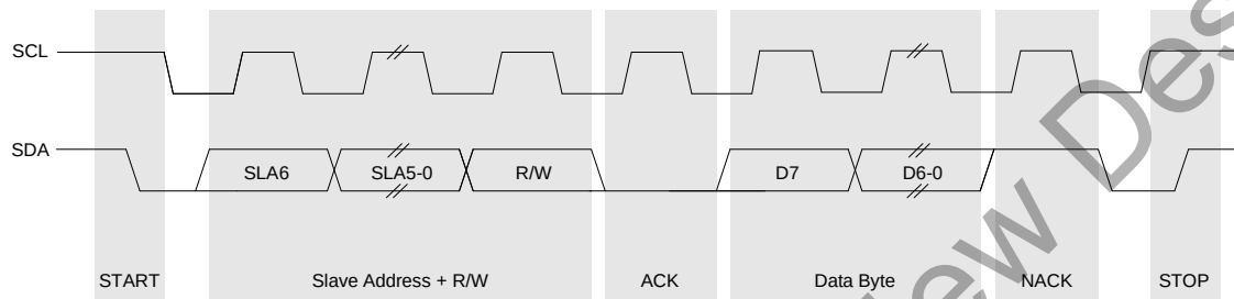
Figure 24.3. SMBus Transaction
