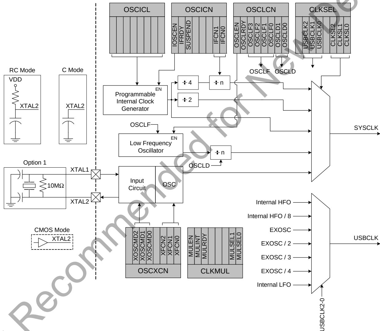
Figure 21.1. Oscillator Options
