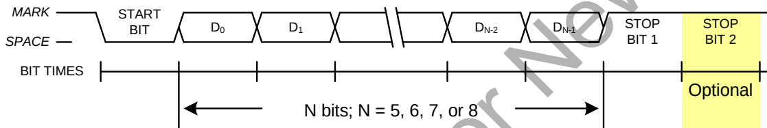
Figure 26.2. UART1 Timing Without Parity or Extra Bit
