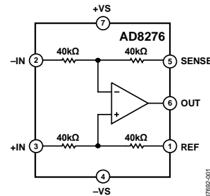
Figure 1. AD8276
