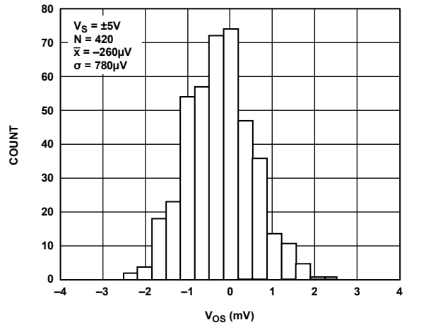
Figure 35. Input Offset Voltage Distribution
