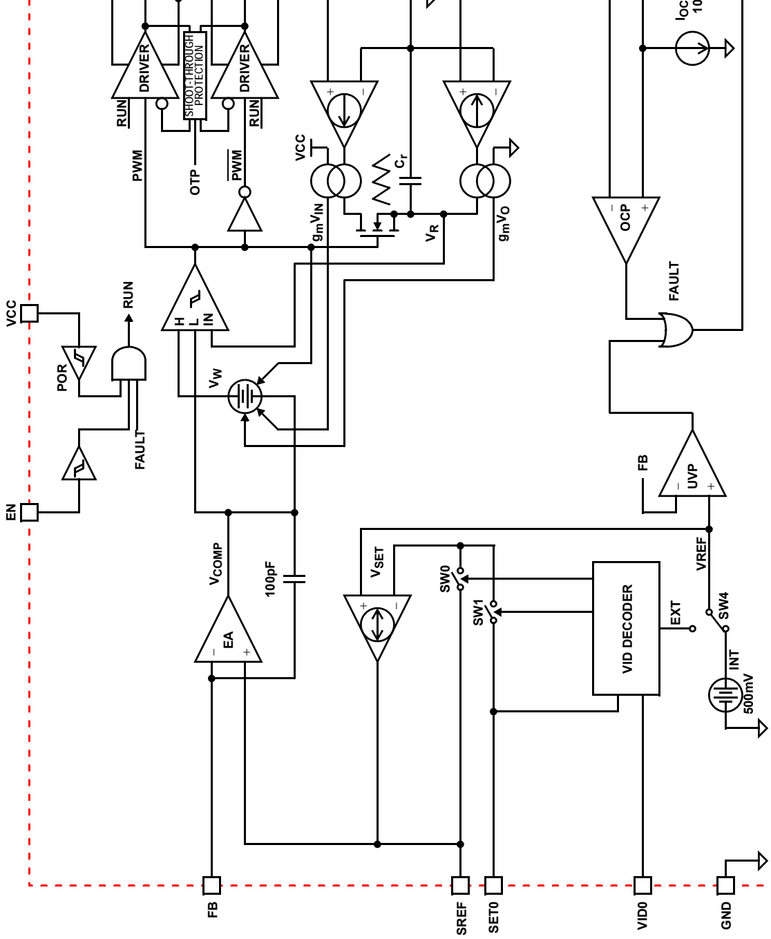
FIGURE 1. SIMPLIFIED FUNCTIONAL BLOCK DIAGRAM OF ISL62873
