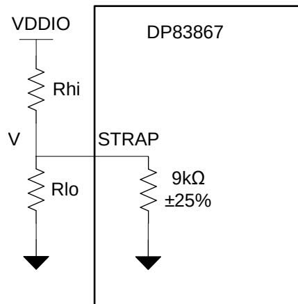
Figure 20. Strap Circuit
