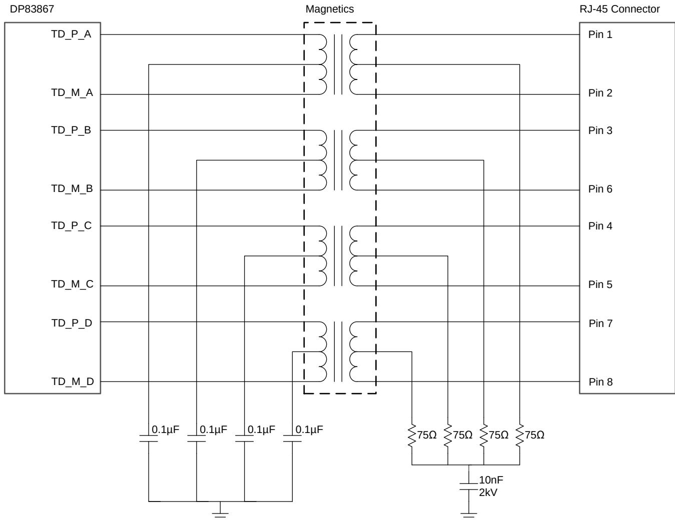
Figure 26. Magnetics Connections
