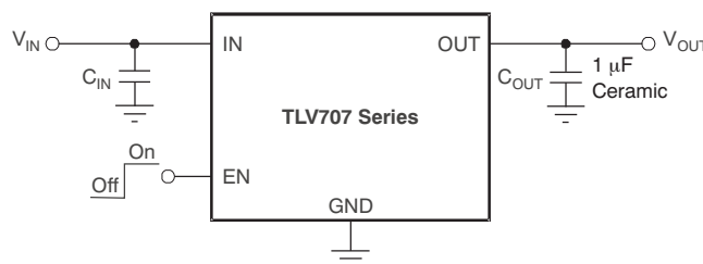
Typical Application Circuit
