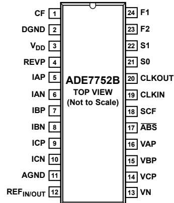
Figure 3. Pin Configuration
