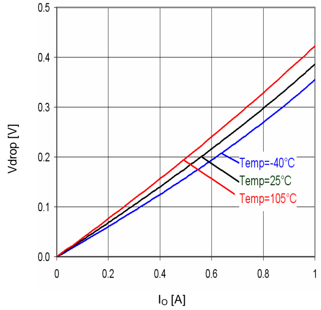
Fig.36 Minimum dropout Voltage 2 (V CC =4V, T a =25°C)
