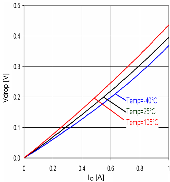
Fig.37 Minimum dropout Voltage 5 (V CC =5.5V, T a =25°C)
