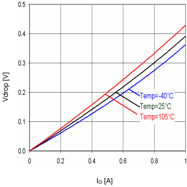
Fig.35 Minimum dropout Voltage 2 (V CC =3.3, T a =25°C)
