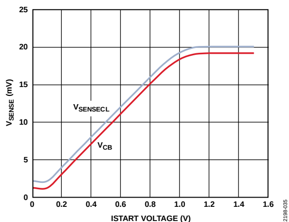
Figure 38. V_{SENSE} vs. ISTART Voltage
