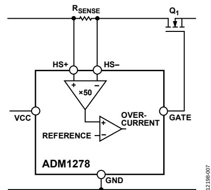
Figure 47. Hot Swap Current Sense Amplifier
