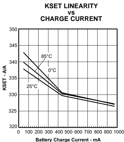
Figure 10. 3.0 < V_{(BAT)} < 4.0 V
