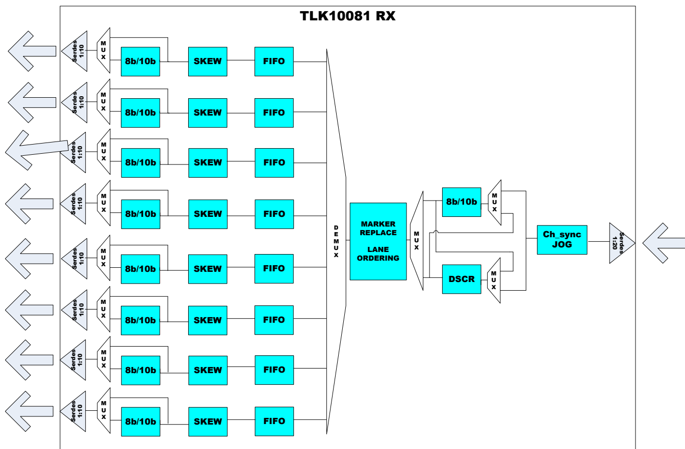
Figure 2-2. A Simplified Block Diagram of the TLK10081 (RX)
