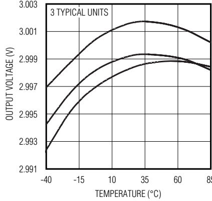
OUTPUT VOLTAGE vs. TEMPERATURE ( V_{OUT} = 3V )
