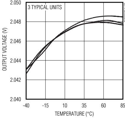
OUTPUT VOLTAGE vs. TEMPERATURE ( V_{OUT} = 2.048V )
