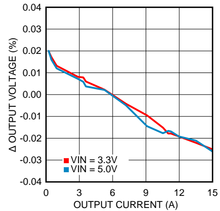
Figure 4. Load Regulation
