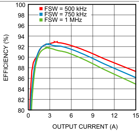
Figure 1. Efficiency
