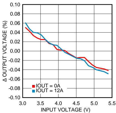
Figure 5. Line Regulation
