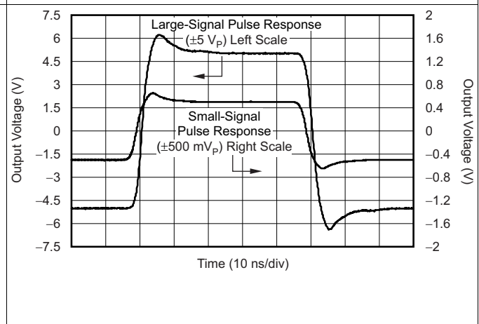
Figure 46. Pulse Response
