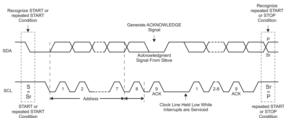
Figure 44. Bus Protocol
