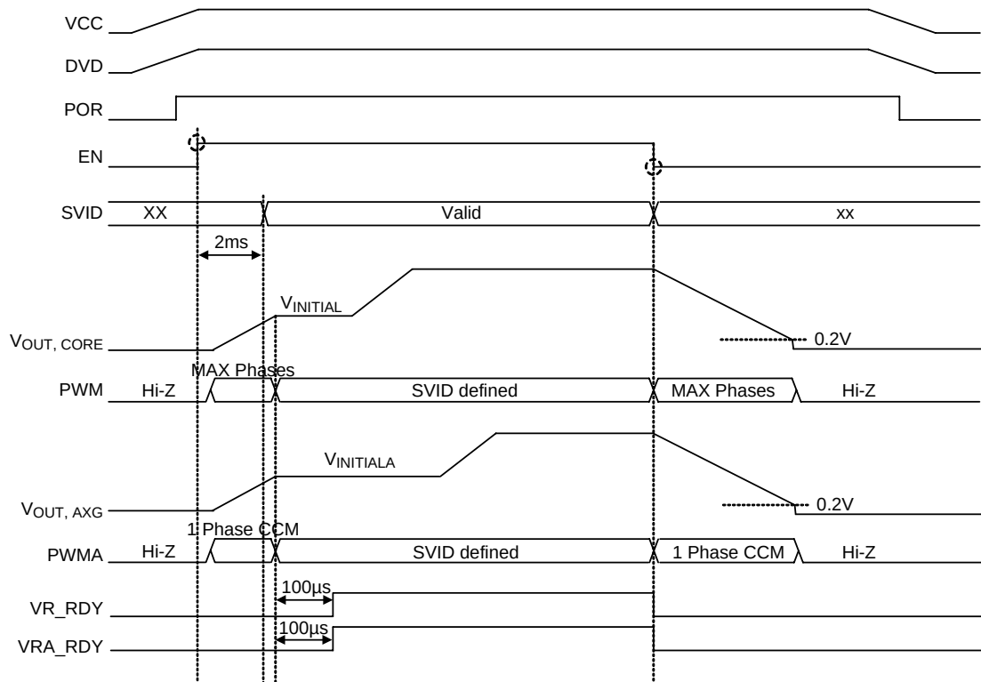
Figure 4 (b). Power Sequence for the RT8859M ( V_{\text{INITIAL}} \neq 0\text{V} , V_{\text{INITIALA}} \neq 0\text{V} )
