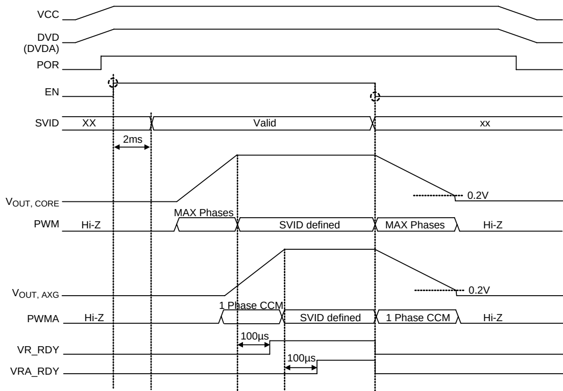
Figure 4 (a). Power Sequence for the RT8859M ( V_{\text{INITIAL}} = V_{\text{INITIALA}} = 0\text{V} )
