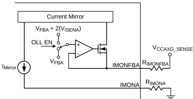
Figure 22. AXG VR : Current Monitoring Circuit
