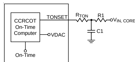
Figure 8. CORE VR : On-Time Setting with R_C Filter
