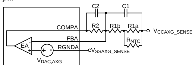
Figure 17. AXG VR : Loop Setting with Temperature Compensation
