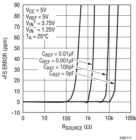
Figure 11. +FS Error vs R_{\text{SOURCE}} at \text{REF}^+ or \text{REF}^- (Small C_{\text{REF}} )
