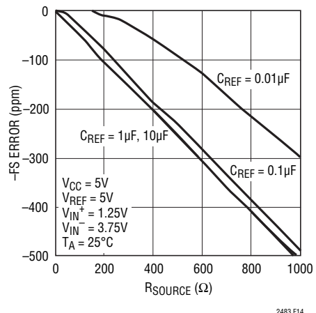
Figure 14. -FS Error vs R_{\text{SOURCE}} at \text{REF}^+ or \text{REF}^- (Large C_{\text{REF}} )
