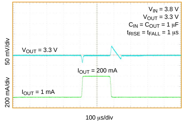
Figure 20. Load Transient Response, 1 mA – 200 mA NCV8752A/B, V_{OUT} = 3.3 V
