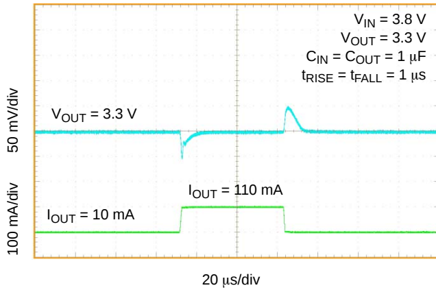
Figure 17. Load Transient Response, 10 mA – 110 mA NCV8752A/B, V_{OUT} = 3.3 V
