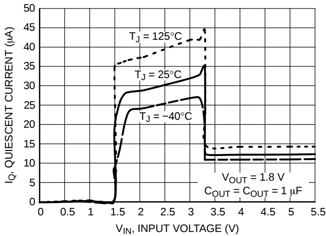
Figure 63. Quiescent Current vs. Input Voltage V_{OUT} = 1.8\text{ V}
