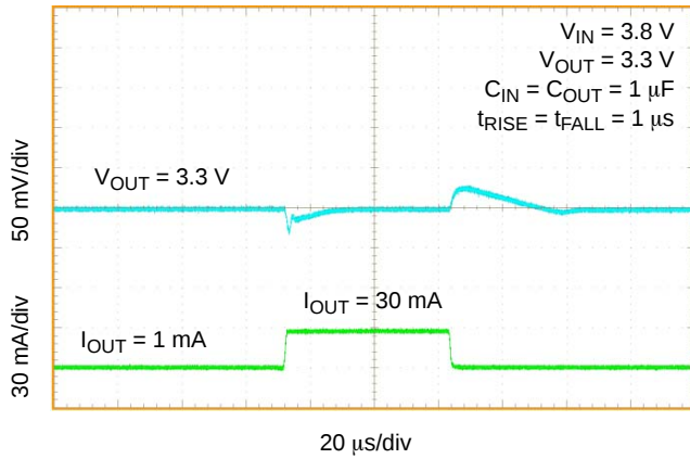
Figure 15. Load Transient Response, 1 mA – 30 mA NCV8752A/B, V_{OUT} = 3.3 V
