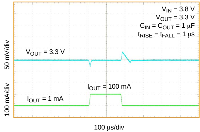
Figure 16. Load Transient Response, 1 mA – 100 mA NCV8752A/B, V_{OUT} = 3.3 V
