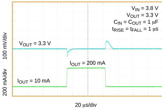
Figure 19. Load Transient Response, 10 mA – 200 mA NCV8752A/B, V_{OUT} = 3.3 V
