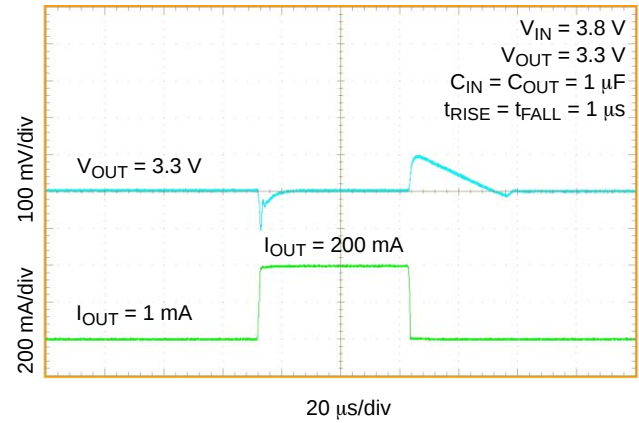
Figure 18. Load Transient Response, 1 mA – 200 mA NCV8752A/B, V_{OUT} = 3.3 V
