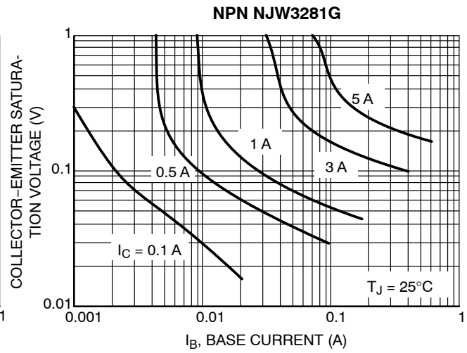
Figure 8. Saturation Region
