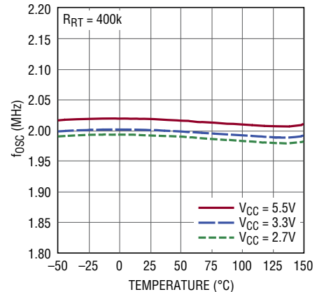
RT Programmed Oscillator Frequency vs Temperature
