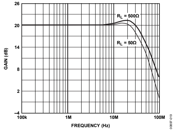
Figure 19. Gain vs. Frequency, Gain = -10
