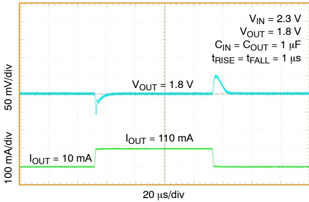
Figure 11. Load Transient Response, 10 mA – 110 mA NCP752A/B, V_{OUT} = 1.8\text{ V}
