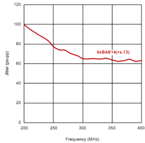
Figure 4. Fractional Divider Input Frequency Impact on Jitter
