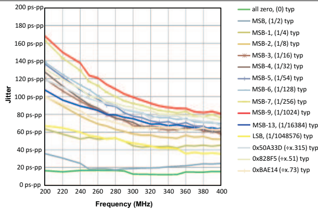
Figure 3. Fractional Divider Bit Selection Impact on Jitter
