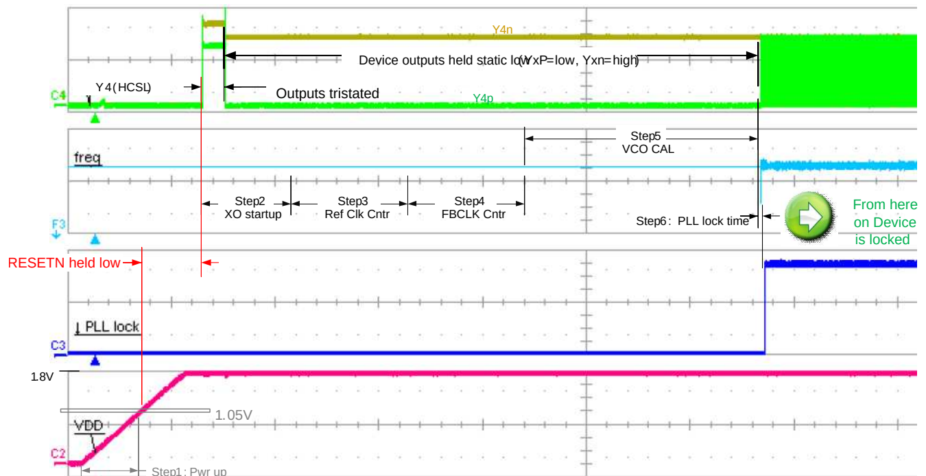
Figure 41. Powerup Time
