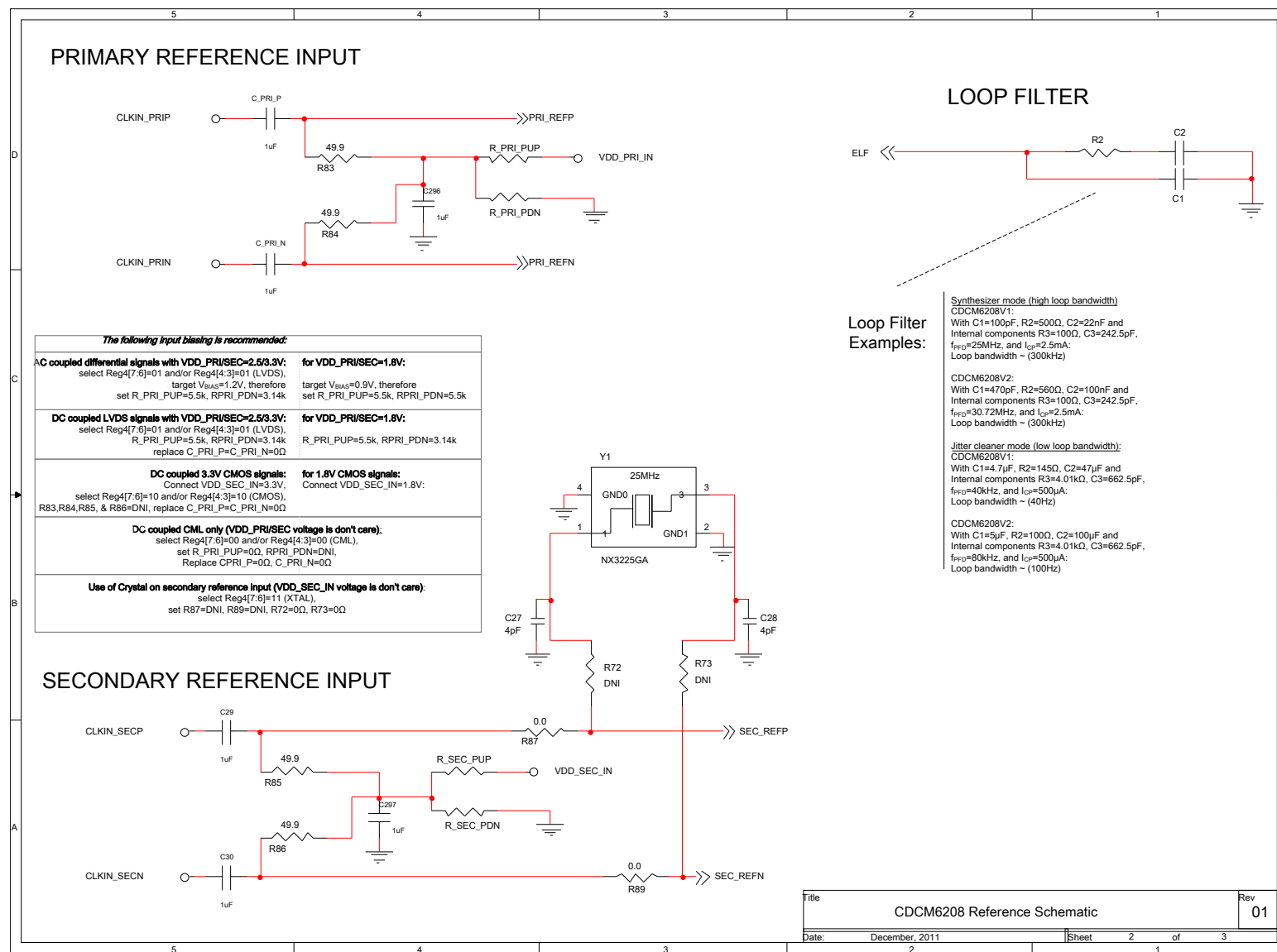
Figure 61. Schematic Page 2
