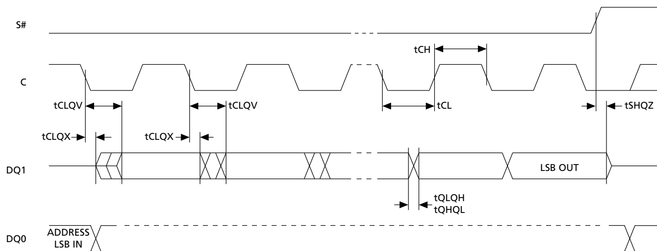
Figure 31: Output Timing
