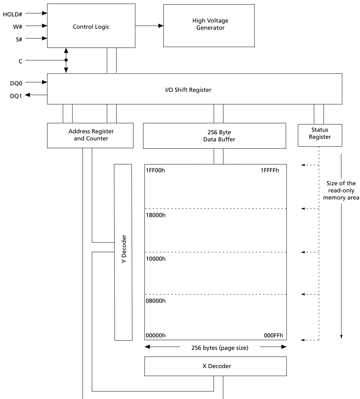
Figure 6: M25PE10 Block Diagram
