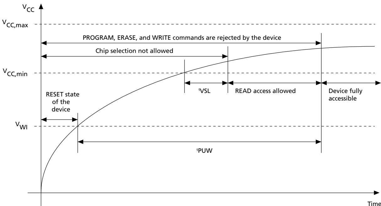
Figure 27: Power-Up Timing
