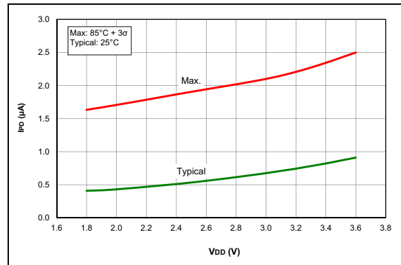
FIGURE 33-35: I_{PD} , Watchdog Timer (WDT). PIC16F1704/8 Only.
