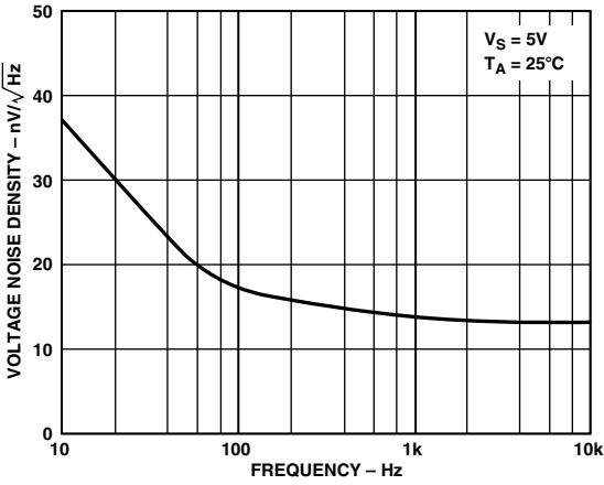
Figure 13. Voltage Noise Density vs. Frequency
