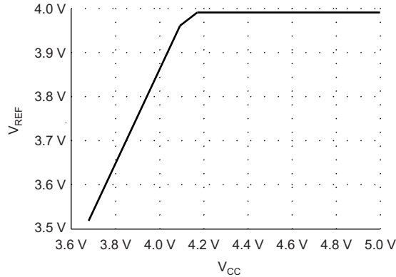
Figure 14. UCC3813-3 REF Output vs V VCC
