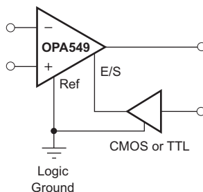
Figure 5. Output Disable
