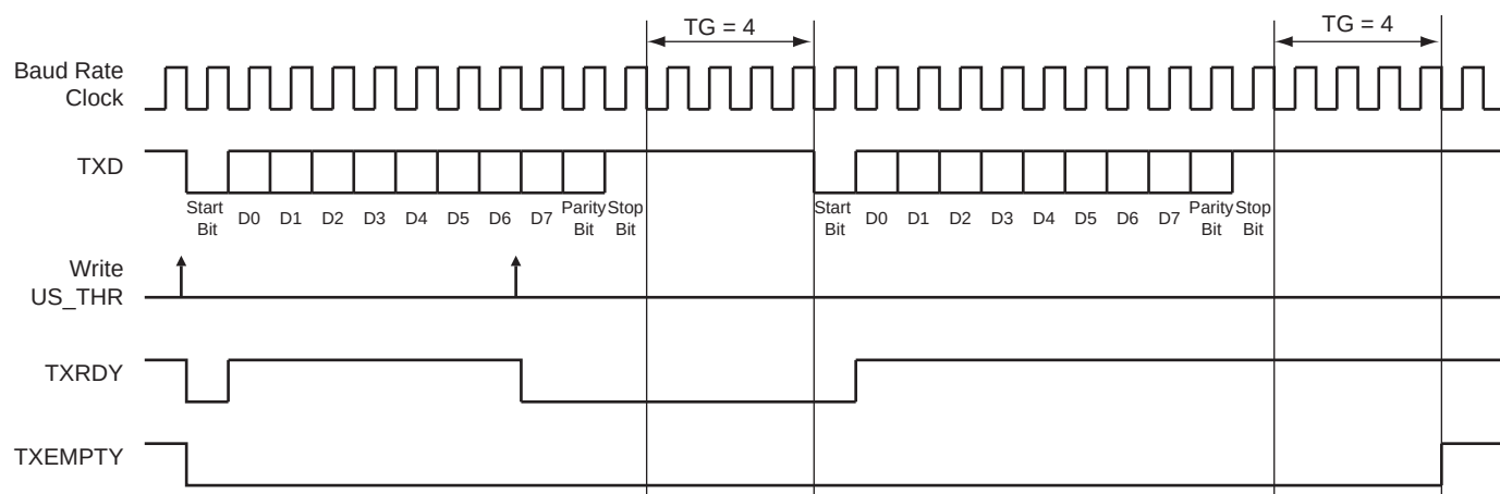
Figure 37-22. Timeguard Operations
