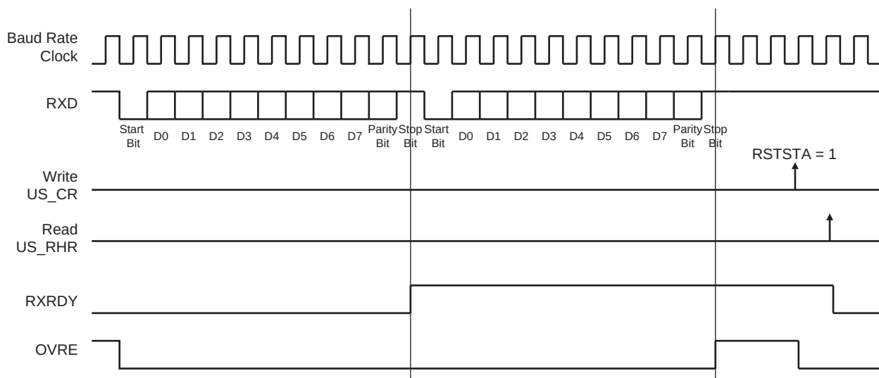
Figure 37-20. Receiver Status
