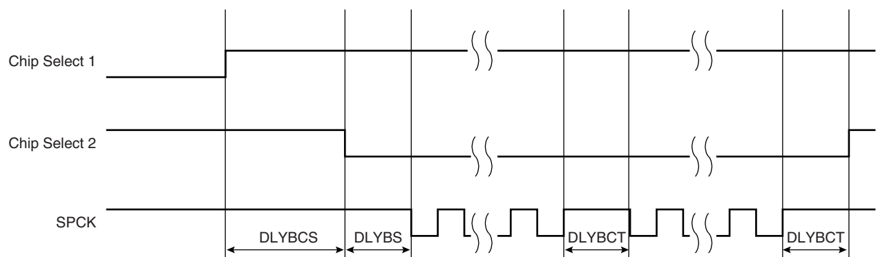
Figure 20-7. Programmable Delays
