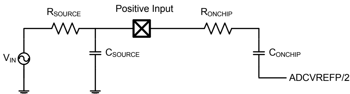
Figure 32-7. ADC Input
