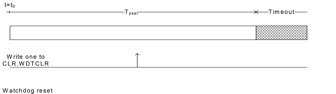
Figure 15-2. Basic Mode WDT Timing Diagram, normal operation.
