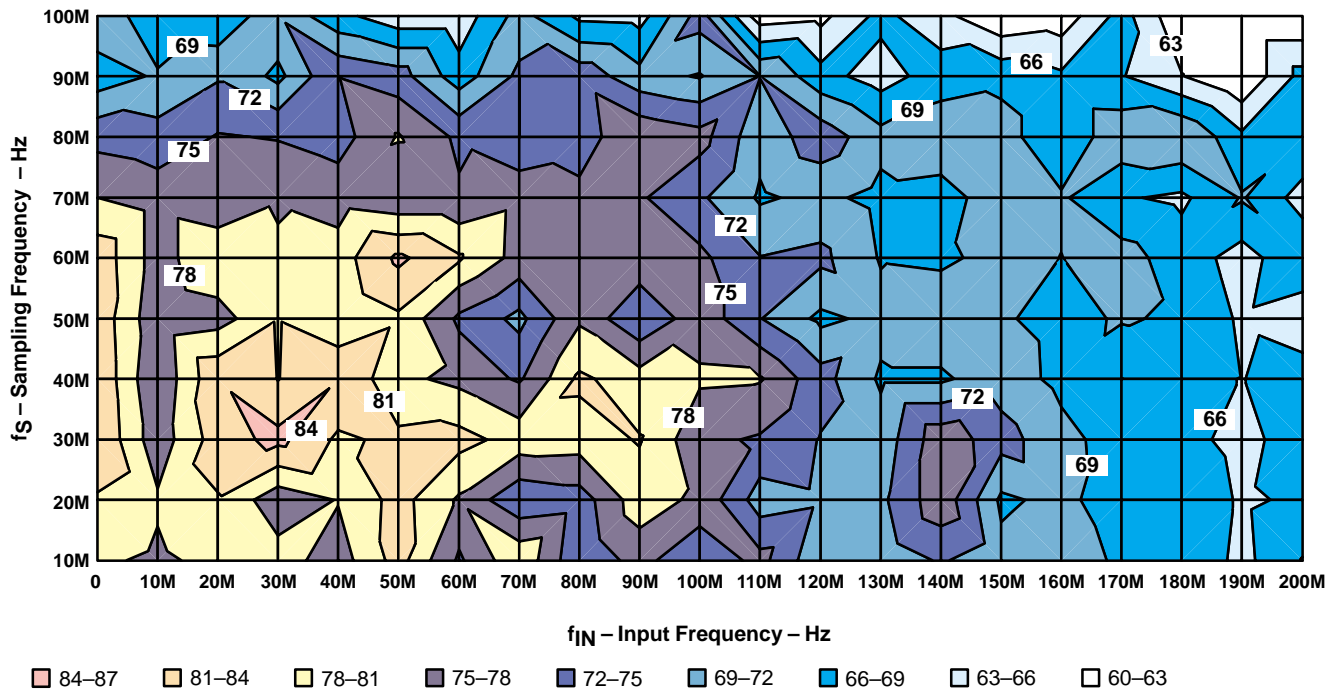
Figure 9. SFDR [dBc]
