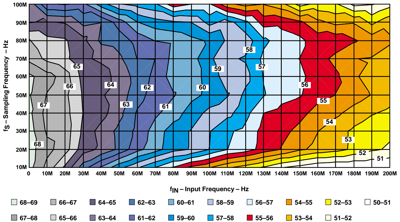
Figure 8. SINAD [dBFS]
