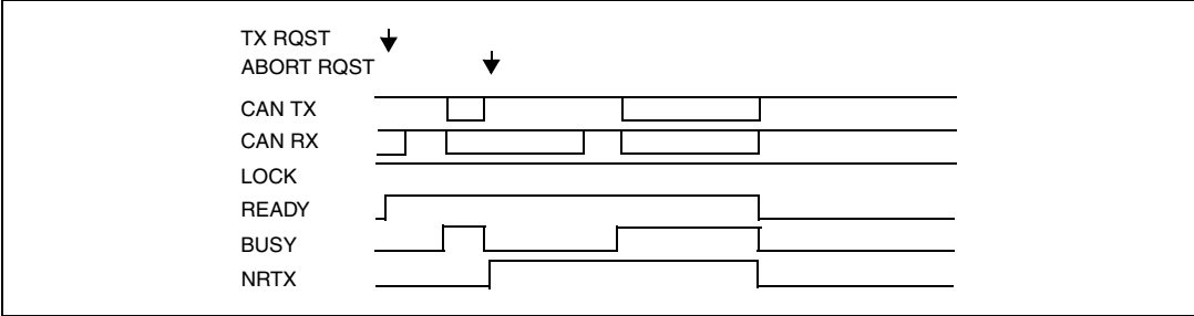
Figure 83. Abort with the software workaround - by NRTX, BUSY and LOCK
