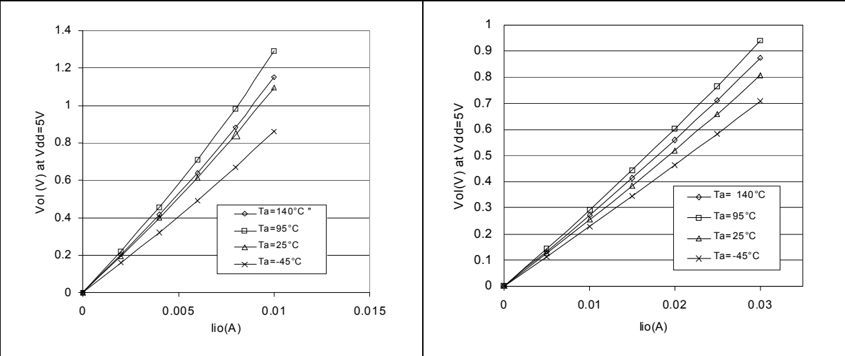
Figure 99. Typical V_{OL} at V_{DD} = 5V (standard) Figure 100. Typical V_{OL} at V_{DD} = 5V (high-sink)
