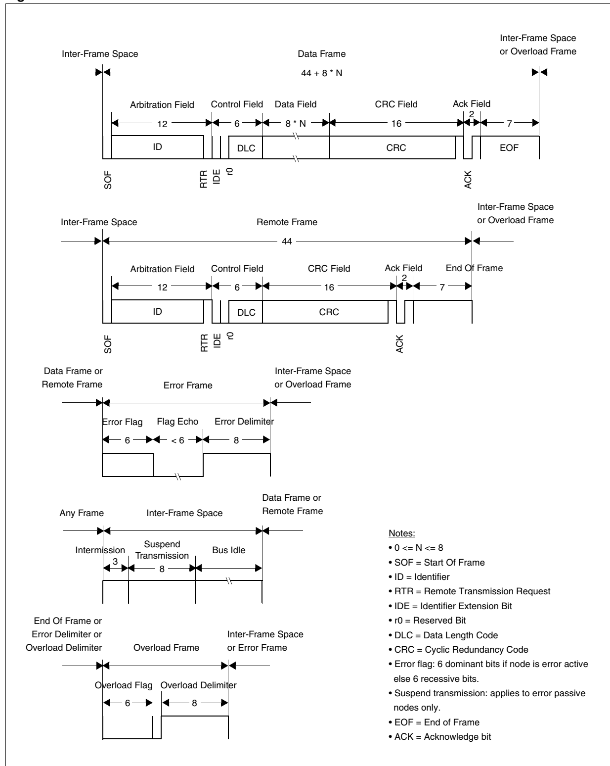
Figure 71. CAN frames
