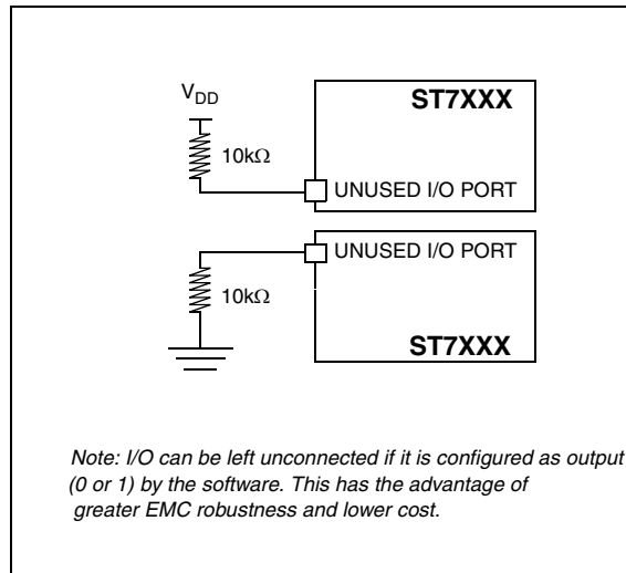
Figure 97. Unused I/O pins configured as input
