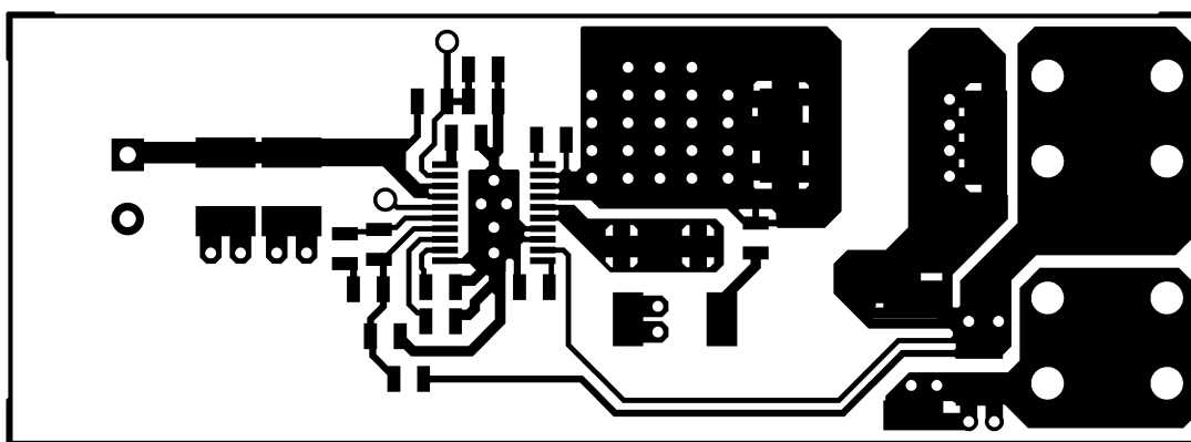
Figure 29. Component Side
