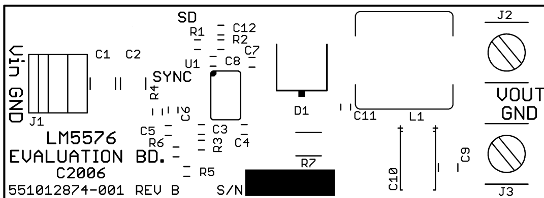
Figure 28. Silkscreen
