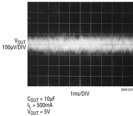
10Hz to 100kHz Output Noise, C_{BYP} = 1000\text{pF}
