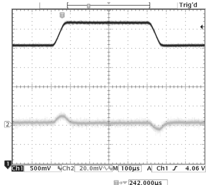
Figure 17. Line Transient (LDO1)
