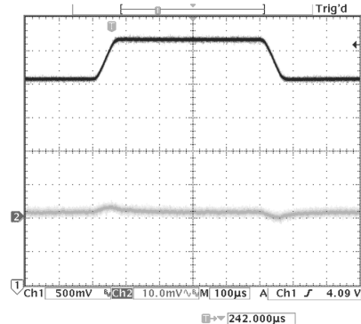
Figure 18. Line Transient (LDO2)
