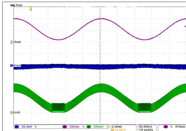
Figure 37. PWM-PSM-Transition
