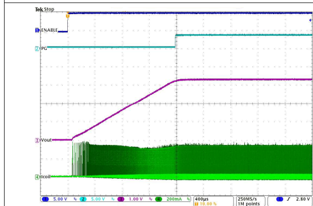
Figure 41. Start Up into 100 mA
