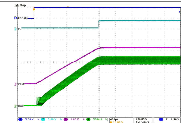
Figure 42. Start Up into 3 A
