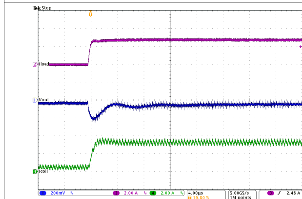
Figure 39. Load Transient Response of Figure 38, Rising Edge
