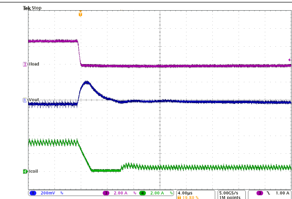
Figure 40. Load Transient Response of Figure 38, Falling Edge
