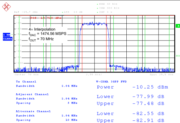
Figure 29. Single-Carrier WCDMA Test Mode1
