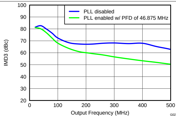
Figure 21. IMD3 vs Output Frequency Over Clamping Options
