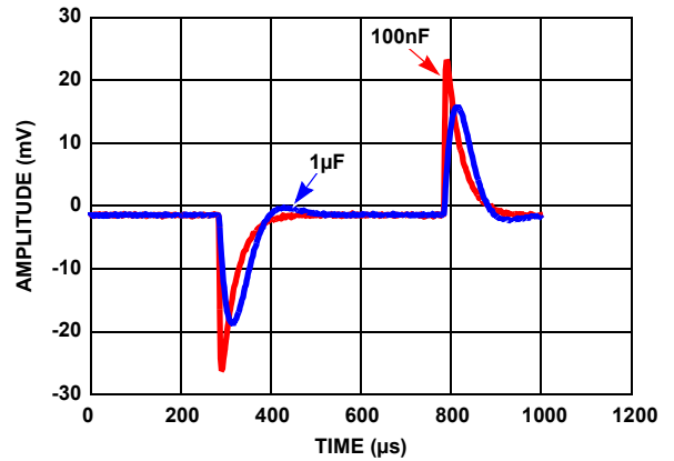
FIGURE 10. LOAD TRANSIENT ( \Delta I_{LOAD} = \pm 1\text{mA} )
