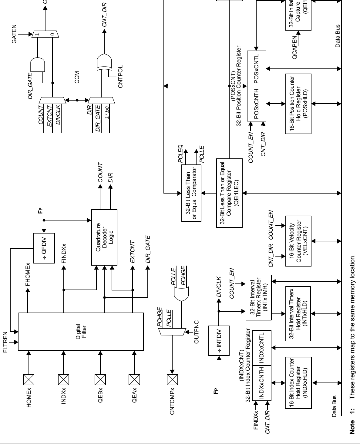
FIGURE 17-1: QEix BLOCK DIAGRAM
