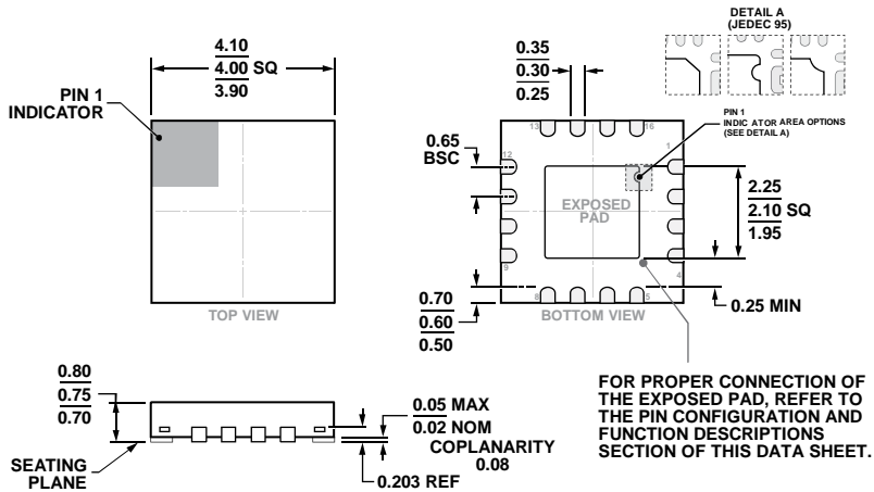
COMPLIANT TO JEDEC STANDARDS MO-220-WGGC. Figure 37. 16-Lead Lead Frame Chip Scale Package [LFCSP] 4 mm × 4 mm Body and 0.75 mm Package Height (CP-16-23) Dimensions shown in millimeters
