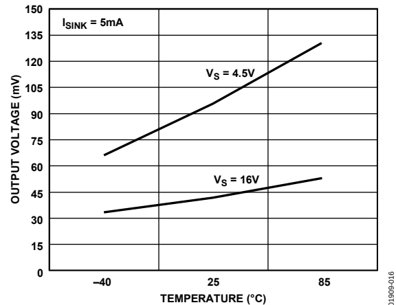
Figure 16. Output Voltage Swing to Rail vs. Temperature
