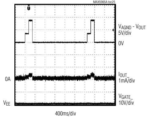
DETECTION WITH MIDSPAN MODE WITH INVALID PD (33kΩ)
