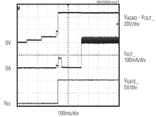
STARTUP IN MIDSPAN MODE WITH VALID PD (25kΩ AND 0.1μF)
