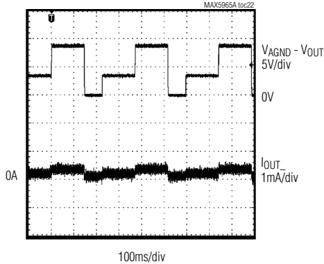
DETECTION WITH INVALID PD (33kΩ)
