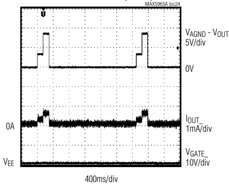
DETECTION WITH MIDSPAN MODE WITH INVALID PD (15kΩ)
