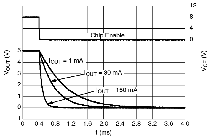
Figure 83. Shutdown, 5.0 V Version D, V_{IN} = 8.0\text{ V}
