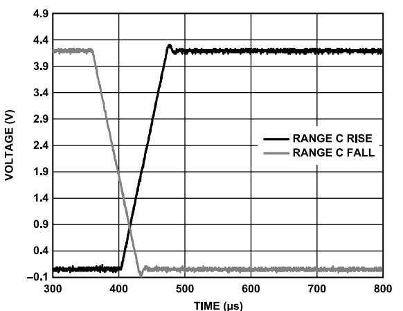
Figure 121. PPMU Force Voltage Transient Response, Range C, 0.0 V to 4.0 V, Uncalibrated, C_{LOAD} = 2000 pF
