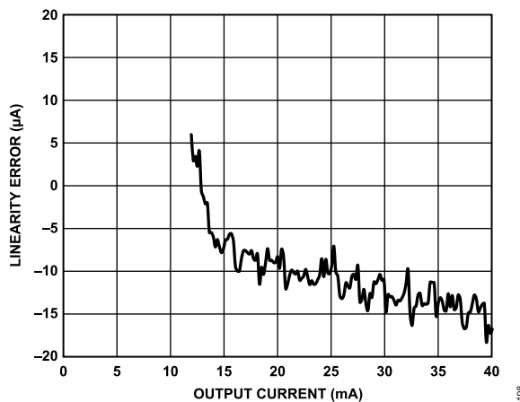
Figure 98. PPMU Current Clamp PCHx INL, Range A
