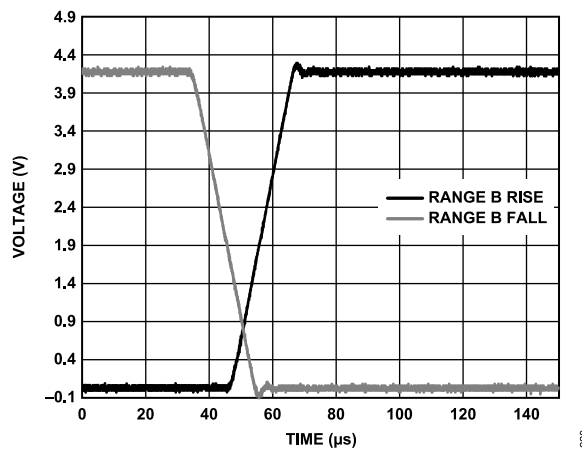
Figure 120. PPMU Force Voltage Transient Response, Range B, 0.0 V to 4.0 V, Uncalibrated, C_{LOAD} = 2000 pF
