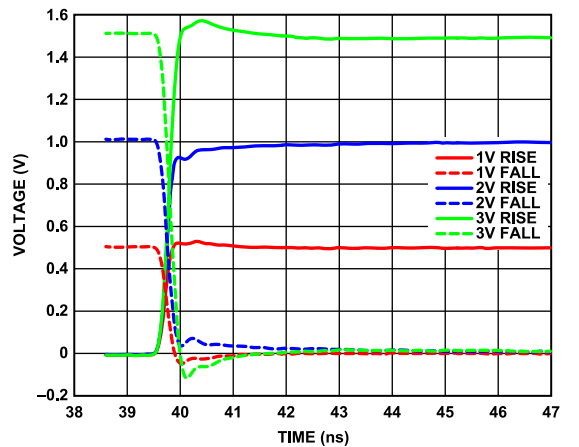
Figure 24. Driver Large Swing Response
