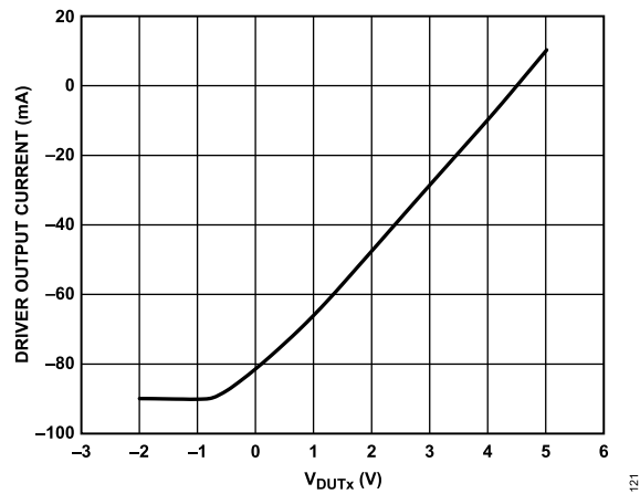
Figure 21. Driver Output Current Limit, Sink
