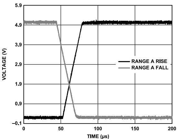
Figure 122. PPMU Force Current Transient Response, Range A, Full-Scale Transition, Uncalibrated, C_{LOAD} = 200 pF, R_{LOAD} = 127 Ω
