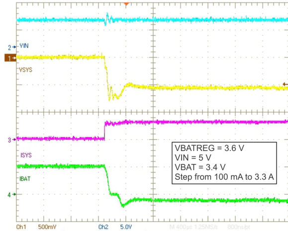
Figure 35. VSYS Transient With Supplement Mode
