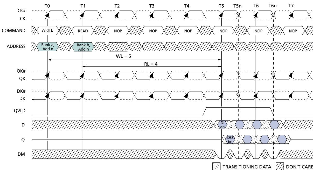
Figure 20: WRITE-to-READ
