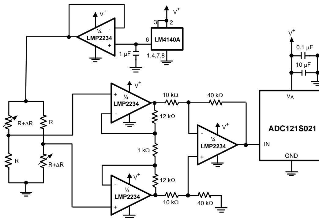
Figure 51. Strain Gauge Bridge Amplifier
