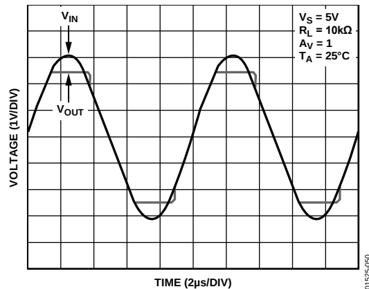
Figure 50. No Phase Reversal
