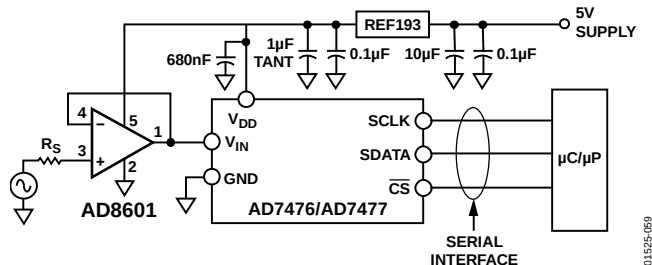
Figure 59. A Complete 3\text{ V} 12-Bit 1\text{ MHz} Analog-to-Digital Conversion System
