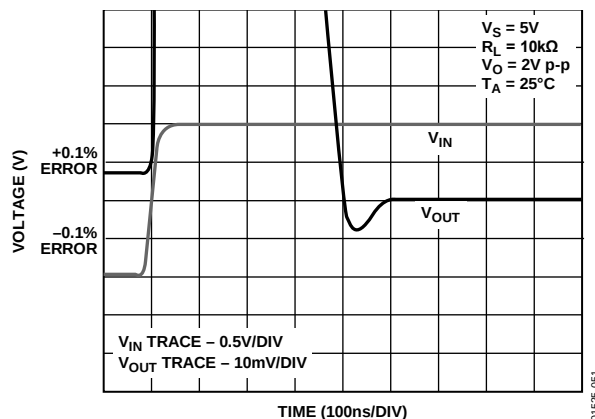
Figure 51. Settling Time
