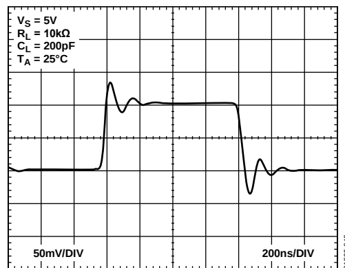
Figure 45. Small Signal Transient Response
